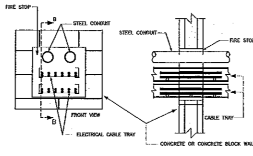
OPENING THROUGH WALL
