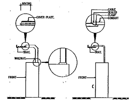
DETAIL FOR RACEWAY AND PANEL CONNECTOR.
