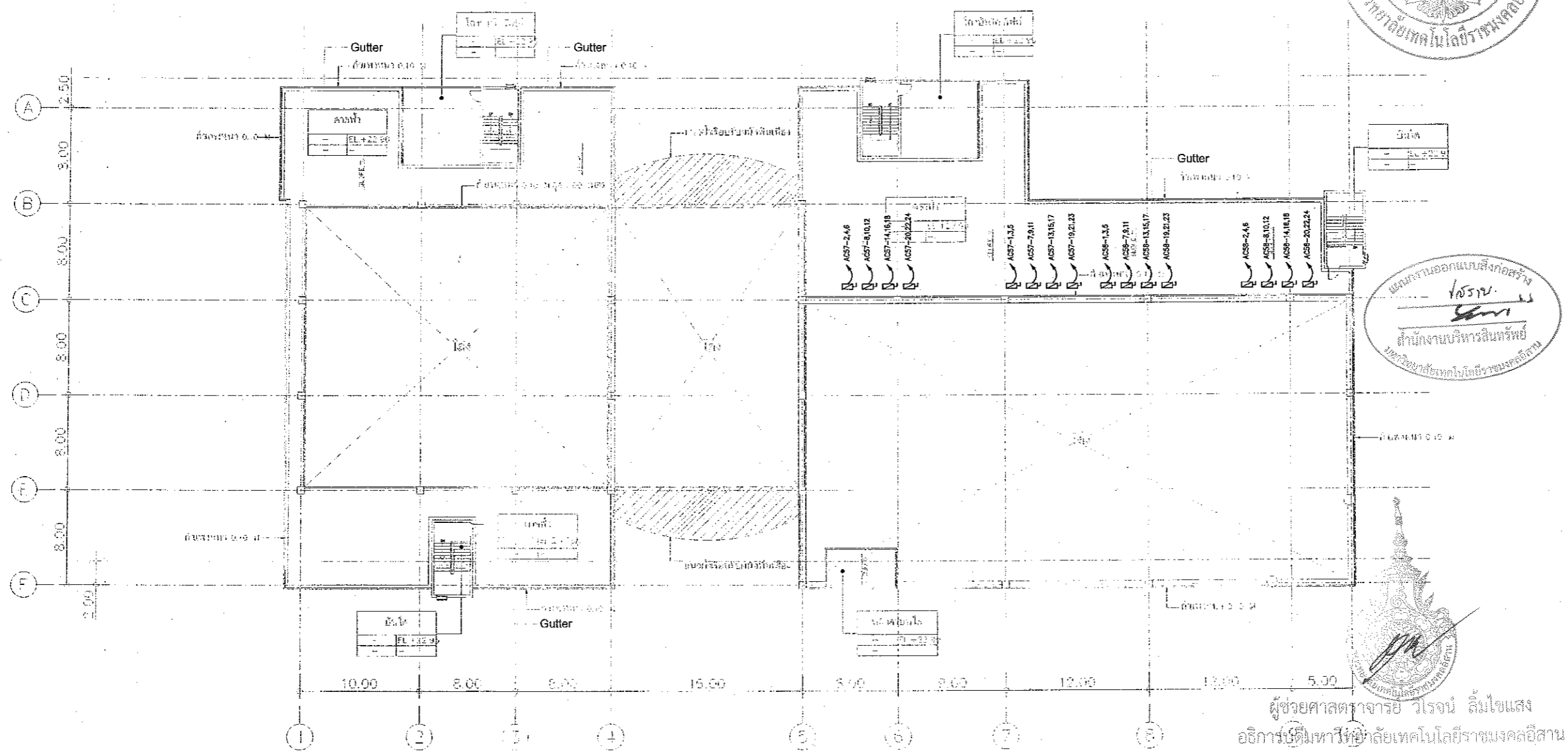
DECK FLOOR PLAN SCALE 1 : 400
