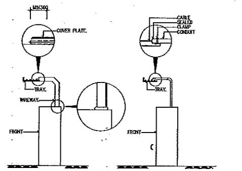
DETAIL FOR RACEWAY AND PANEL CONNECTOR.
