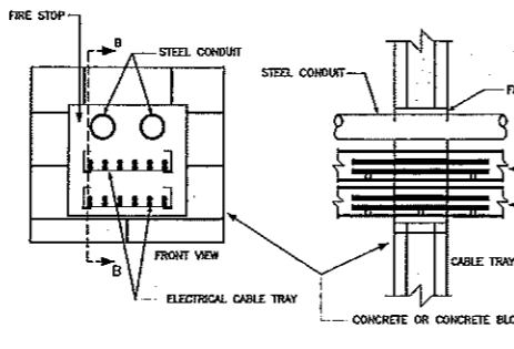
OPENING THROUGH WALL
